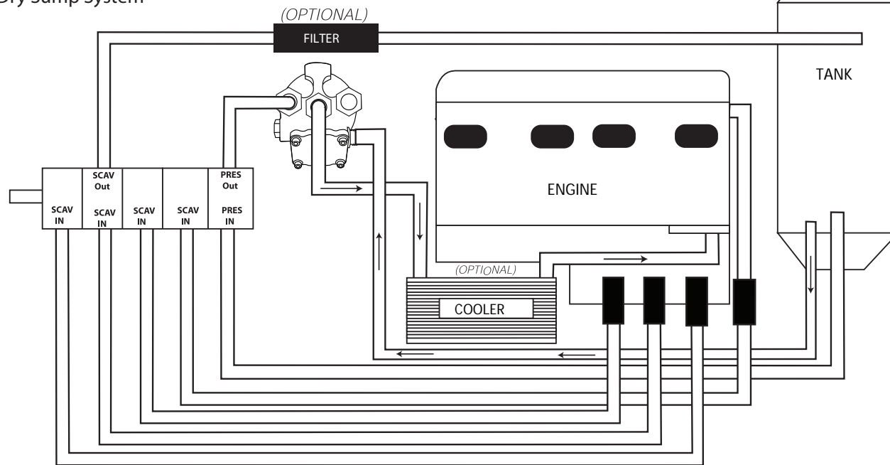
Dry Sump System
